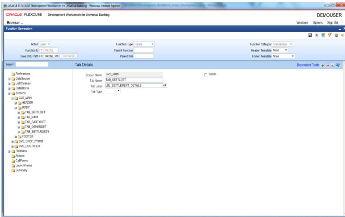
Fig 9.7 Tab Properties
